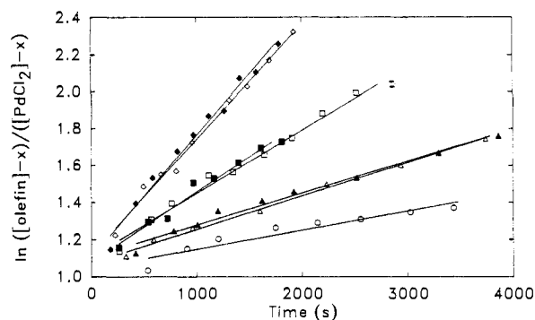
Figure 1. Kinetic plots for reaction of methylenecyclohexane with \text{Na}_2\text{PdCl}_4 in AcOH at 60 (○), 70 (△), 80 (□), and 90 °C (◇).
