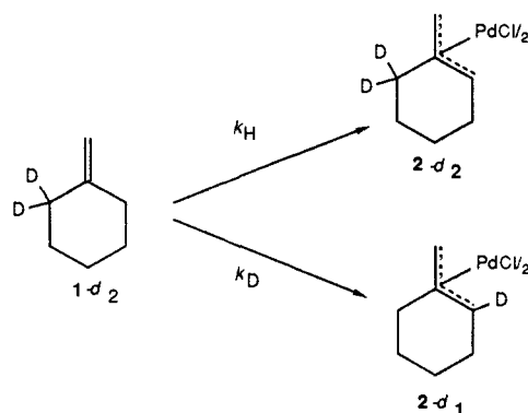
Scheme IV. Determination of the Product Isotope Effect for Allylic Palladation of Methylene-cyclohexane
