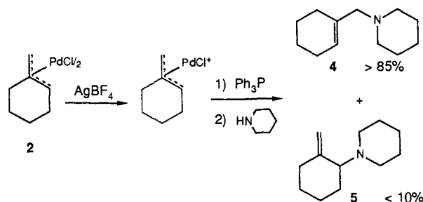
Scheme V. Amination of \pi -Allyl Complex 2
