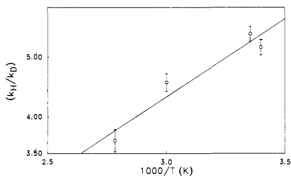
Figure 2. Temperature dependence of k_H/k_D for formation of 2 in DMF solvent. The y axis is \ln scale.
