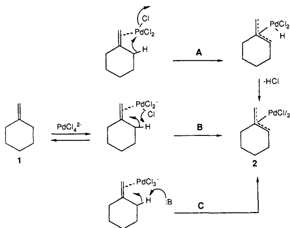
Scheme II. Proposed Mechanisms for (\pi\text{-Allyl})\text{palladium Complex} Formation from Olefins
