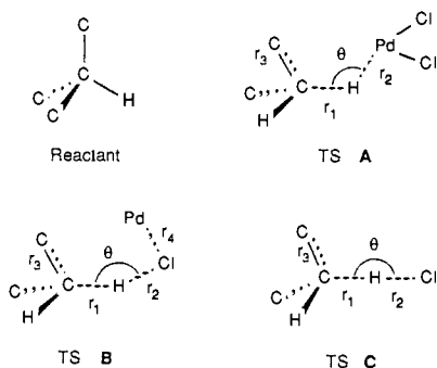
Scheme VI. Cutoff Models of Reactant and Transition States for Isotope Effect Calculations
