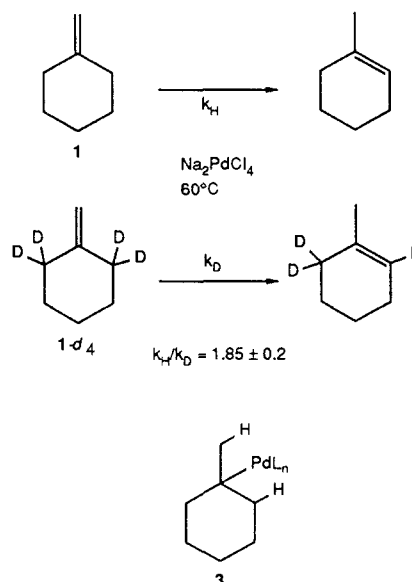
Scheme III. Kinetic Isotope Effect in Pd-Promoted Isomerization of Methylenecyclohexane
